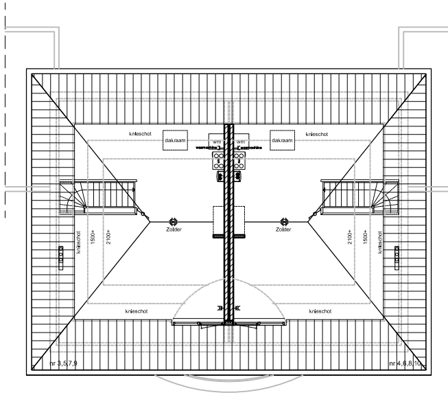
Zolder
